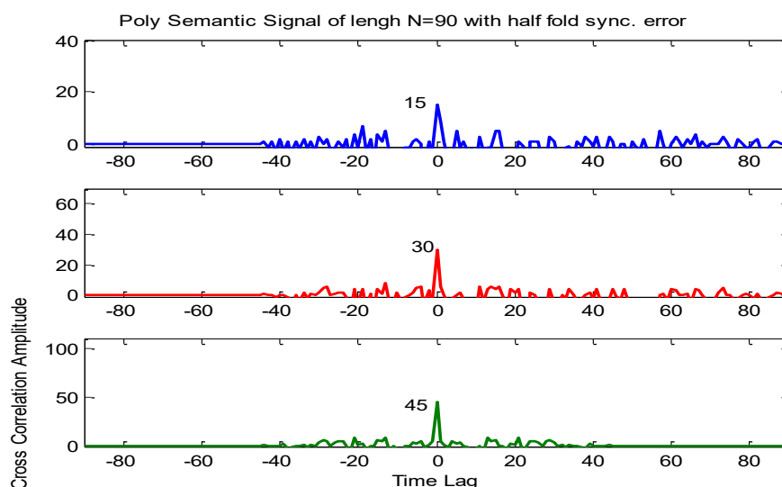
Fig.3 Poly-semantic sequence of length 90 with half fold synchronization bit errors.
