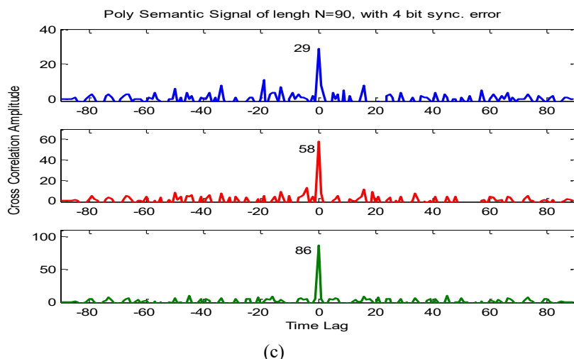
Fig.2 Poly-semantic sequence of length 90 with synchronization error of (a) 1 bit (b) 3 bit (c) 4 bit.
