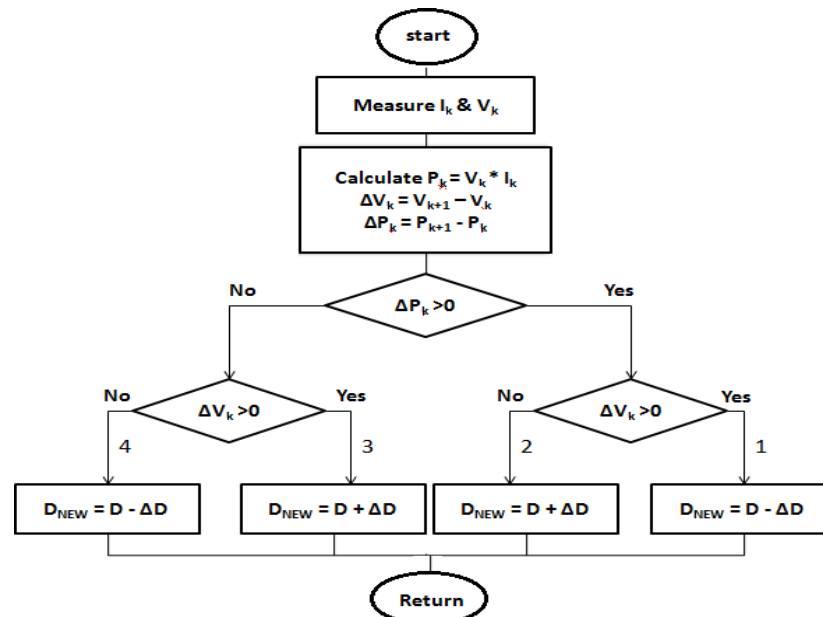
Figure 3.4: P&O strategy
