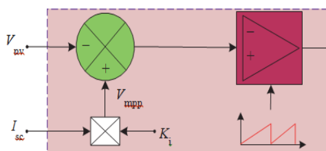
Figure 2.2: Block diagram of ARV MPPT technique
