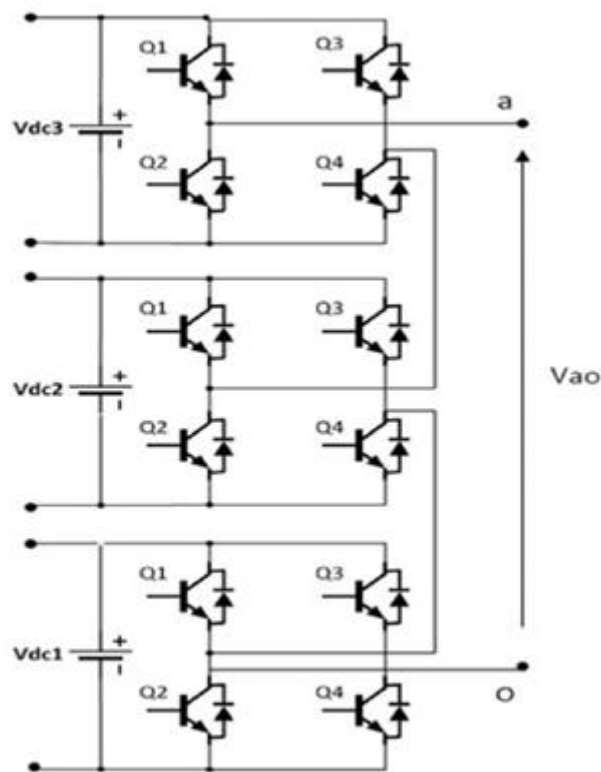
Figure 1 topology of seven level inverters
