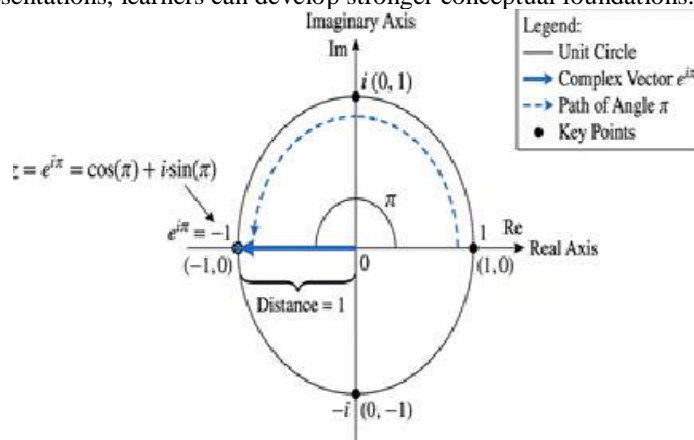
Figure-1-Argand Diagram of Euler's Identity
