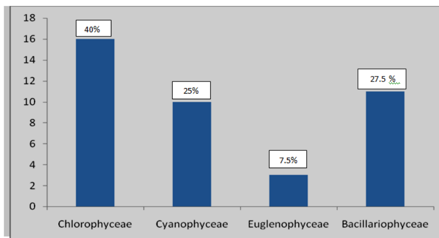
Fig.1: Phytoplankton Total Distribution in Ogane-Aji River
