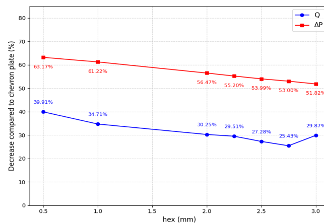
Fig.6: Decrease in heat transfer rate and pressure drop in cylindrical extrusion plate compared to chevron plate
