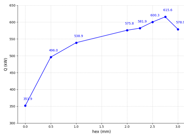
Fig.7: Heat transfer rate vs. extrusion height
