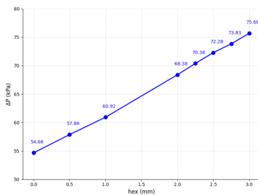
Fig.8: Pressure drop vs. extrusion height
