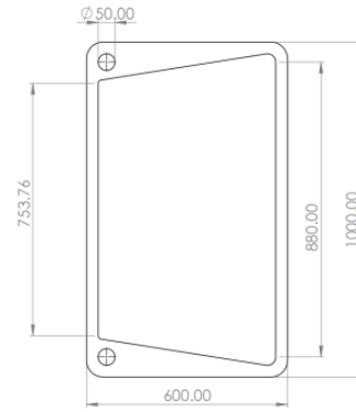
Fig. 4. Gasket geometry
