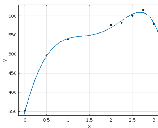
Fig.9: Fitted plot for heat transfer rate
