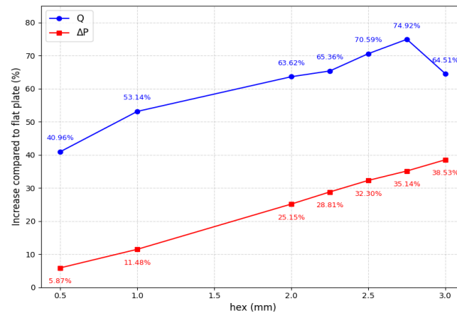
Fig.5: Increase in heat transfer rate and pressure drop in cylindrical extrusion plate compared to flat plate
