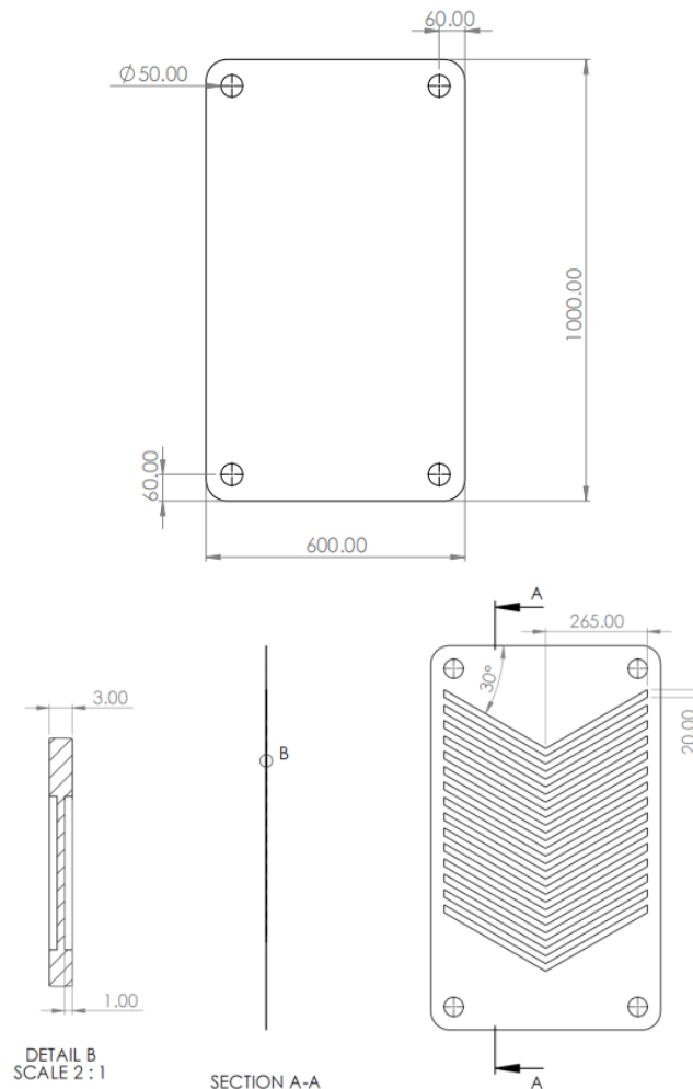
Fig.1: Flat plate geometry
