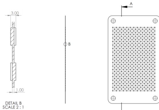
Fig.3: Cylindrical extrusion plate geometry
