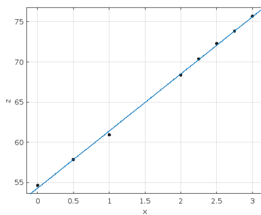
Fig.10: Fitted plot for pressure drop
