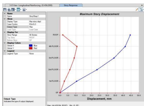
Fig: Maximum Storey Displacement (EQxSLS)
