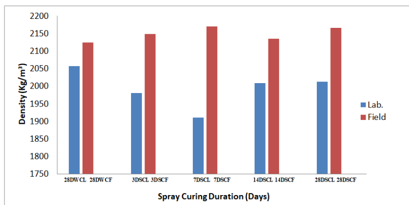
Fig. 5: Average Density Values at 28 Days
