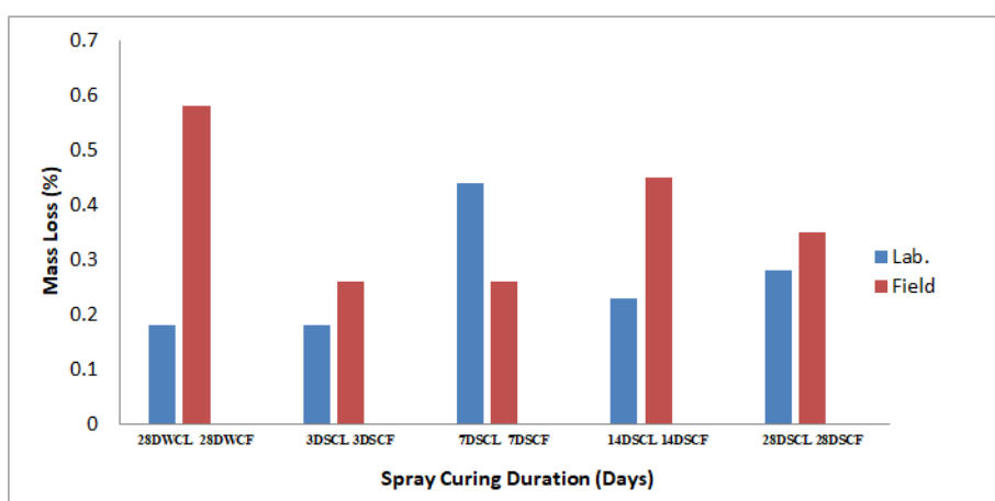
Fig. 6: Average Mass Loss Values at 28 Days
