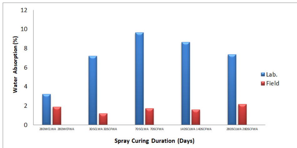
Fig. 8: Average Water Absorption at 28 Days
