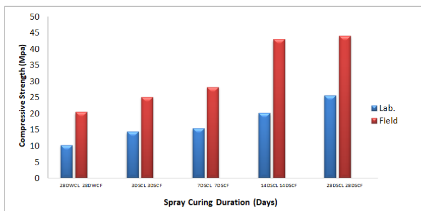
Fig. 7: Average Compressive Strength at 28 Days
