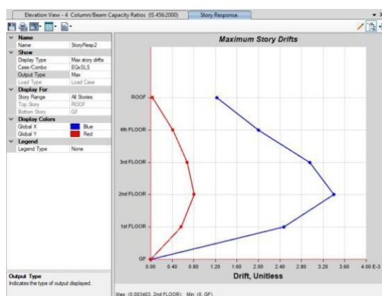
Fig: Maximum Storey Drift (EQySLS)
