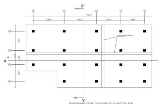
Fig: Reinforcement detail of foundation
