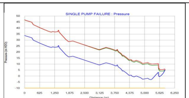
Fig. 4: Pressure variation envelope plot without any surge protection throughout the rising main (Single Pump Failure)
