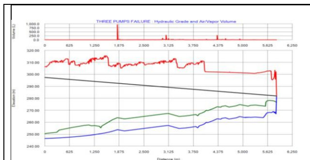
Fig.7: HGL along with Air/Vapor volume variation plot without any surge protection throughout the rising main (Three Pumps Failure)
