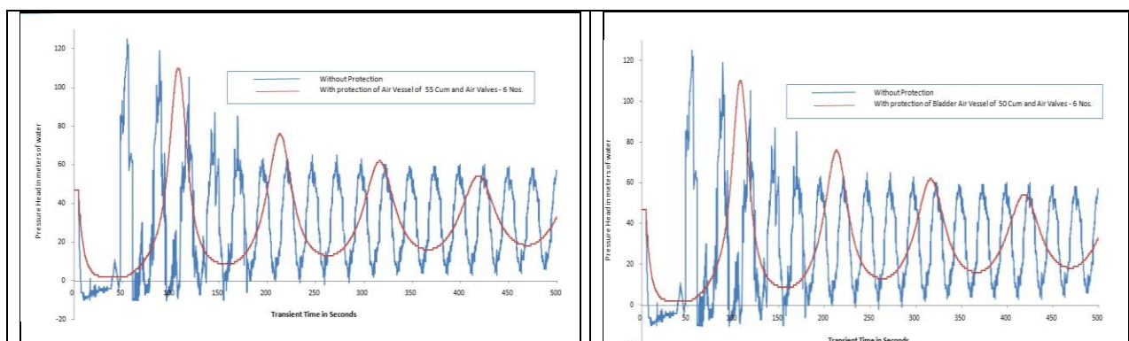
Fig. 21: Pressure variation without and with protection of 50 m 3 capacity compressed air vessel
