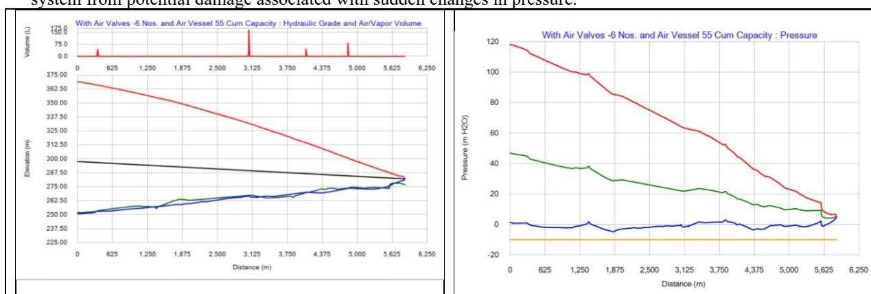
Fig. 13: HGL variation and Air/Vapor volume plot with a surge protection of air vessel of 55 m 3 capacity and air valves -6 Nos. throughout the rising main
