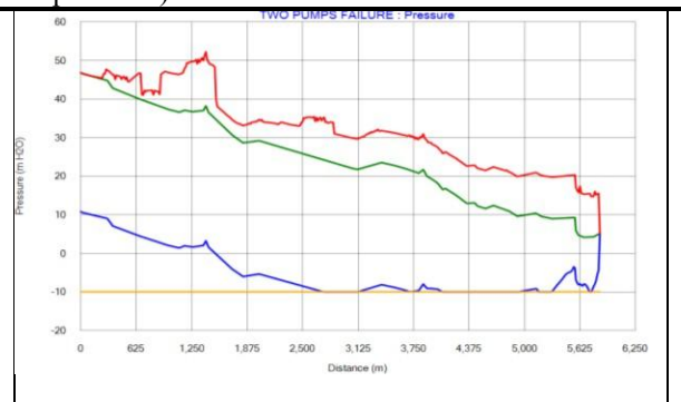
Fig.6: Pressure variation envelope plot without any surge protection throughout the rising main (Two Pumps Failure)
