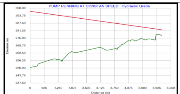
Fig. 2: Steady state hydraulic grade line (HGL) along with pipeline profile
