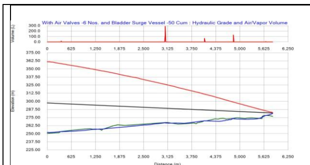
Fig. 17: HGL variation envelope and Air/Vapor volume plot with a bladder surge vessel of 50 m 3 and air valves -6 Nos. throughout the rising main
