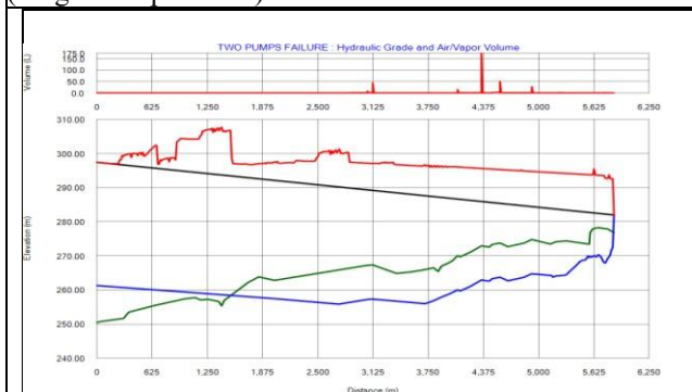
Fig.5: HGL along with Air/Vapor volume variation plot without any surge protection throughout the rising main (Two Pumps Failure)
