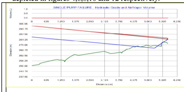
Fig.3: HGL along with Air/Vapor volume variation plot without any surge protection throughout the rising main (Single Pump Failure)
