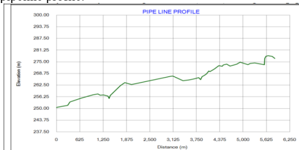
Fig. 1: Rising main profile of Wardha Barrage Lift Irrigation Scheme
