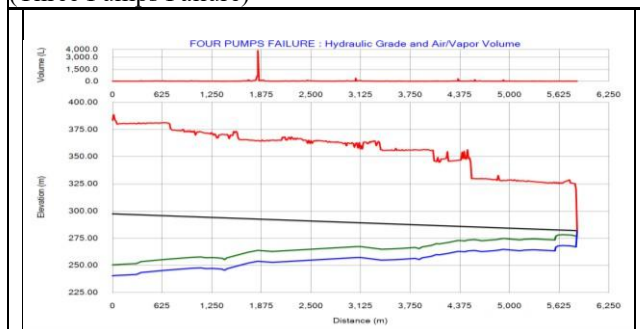
Fig.9: HGL along with Air/Vapor volume variation plot without any surge protection throughout the rising main (Four Pumps Failure)
