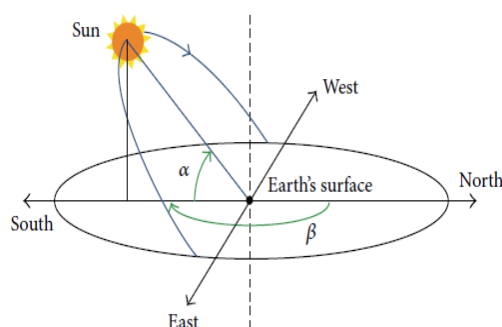
Figure 1: Diagram for solar angles: \alpha - altitude angle, \beta - azimuth angle
