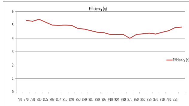
Figure 10: Efficiency V/s Solar Radiation Graph for static plate
