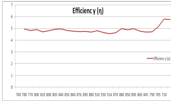
Figure 8: Efficiency V/s Solar Radiation Graph for static plate
