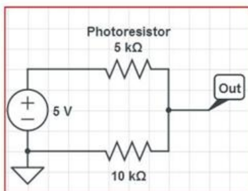
Figure 3: Circuit diagram of Light detection (DDR) sensor
